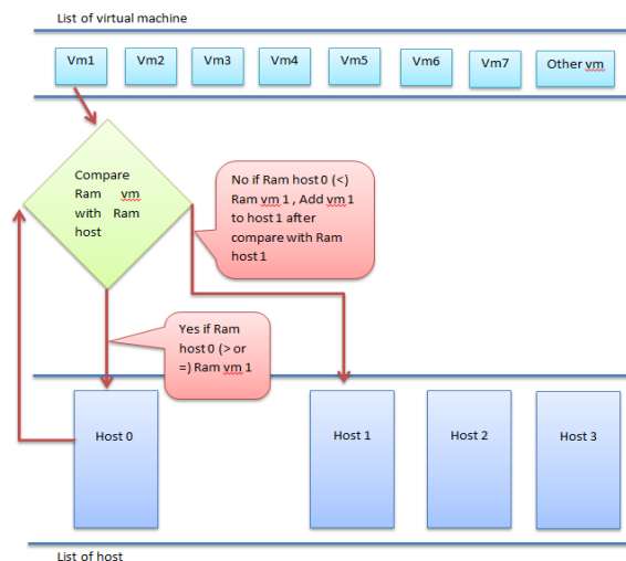
Figure 3: Proposed architecture of algorithm
