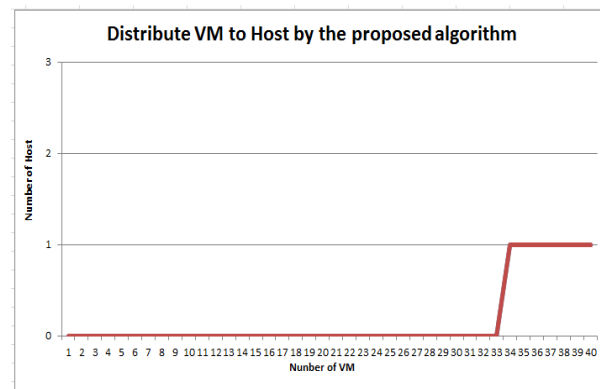
Figure 5: Distribution of VM by proposed algorithm
