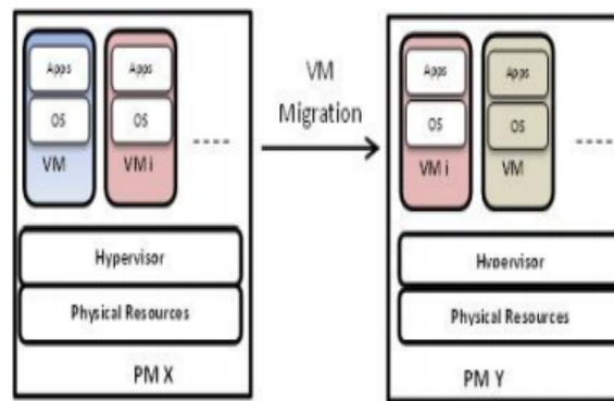
Figure 2: Horizontal Scaling
