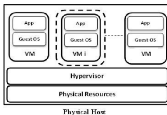
Figure 1: Vertical Scaling
